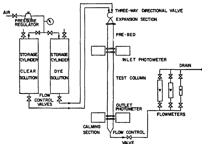
Fig. 1. Flow-system-frequency-response experiments.
