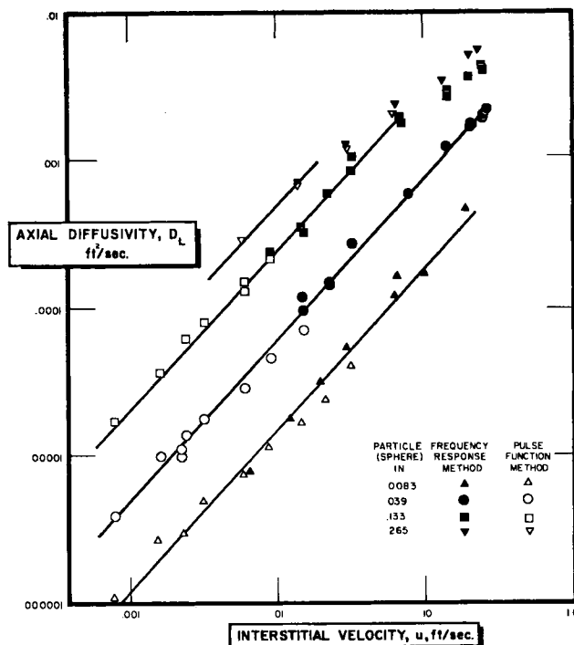
Fig. 6. Dependency of axial diffusivity on particle diameter, plot of C_L = Cd_p^a u^b where D_L = Dd_p^a u^b = C_L u^b .
