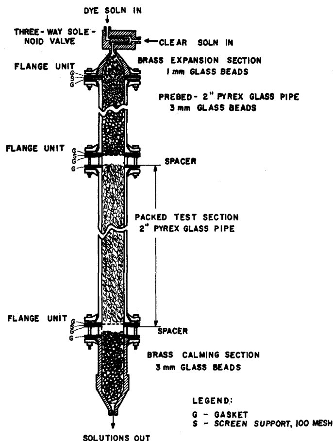
Fig. 2. Column-detail-frequency-response technique.
