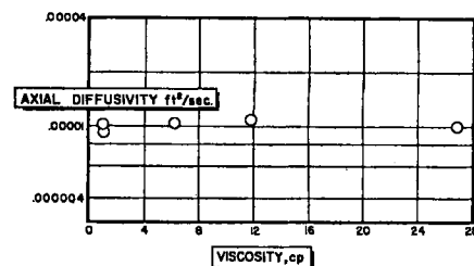
Fig. 8. Pulse function experiment, concentration profile (run P6).
