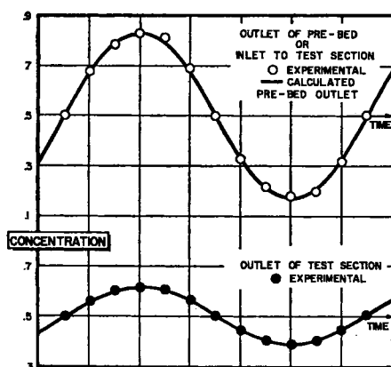
Fig. 3. Periodic sinusoidal waves (run 28). Prebed: 3-mm. spheres, height 1.5 ft.
